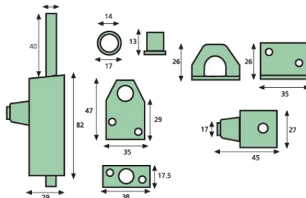
Multi-Purpose Bolt
